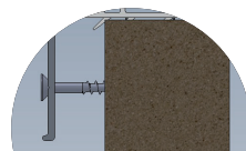
Use fasteners at each pre-drilled location in the frame.
